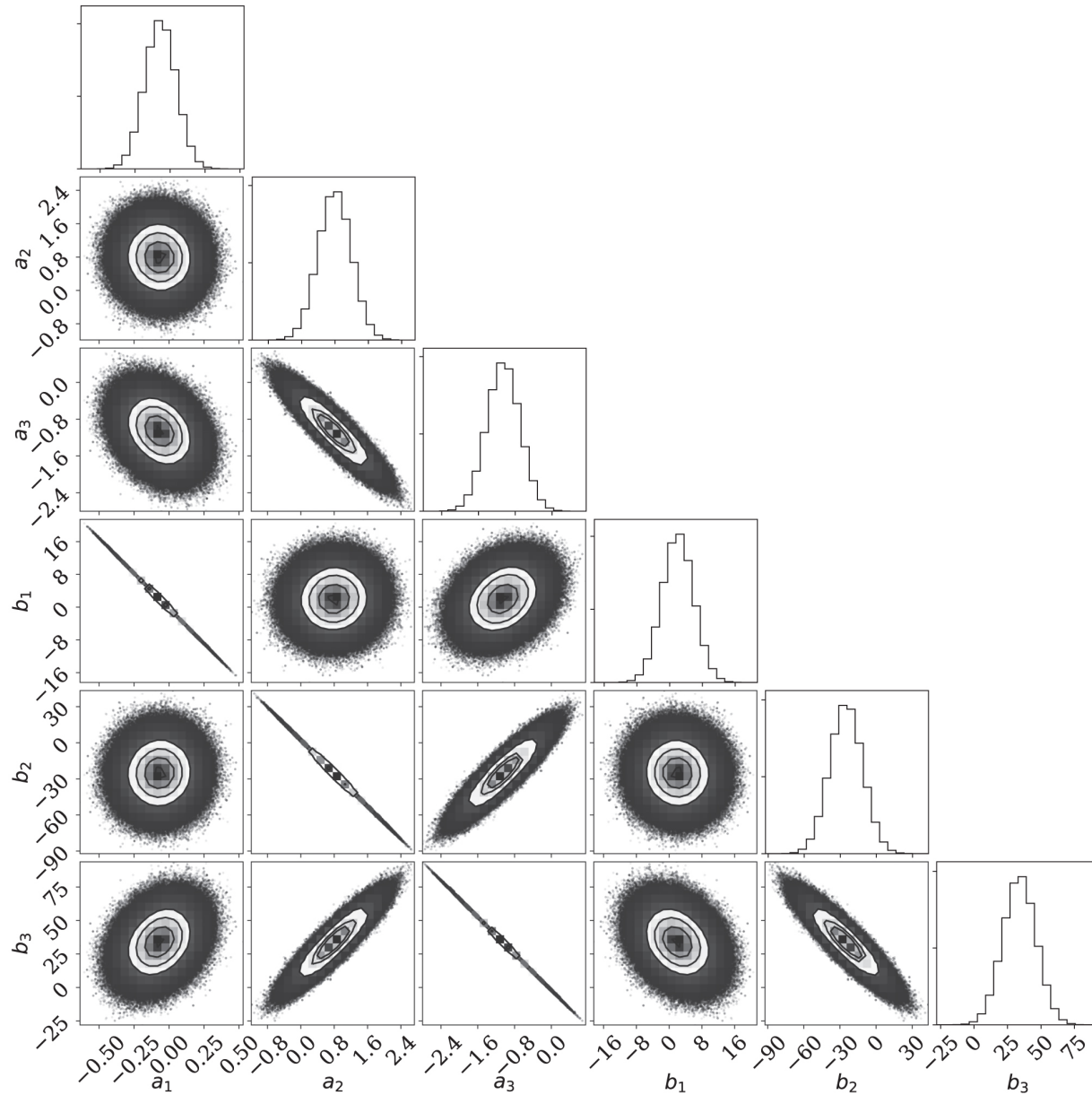
Figure 8. from The Evolution of Flare Activity with Stellar Age null 2019 APJ 871 241 doi:10.3847/1538-4357/aafb76 https://dx.doi.org/10.3847/1538-4357/aafb76 © 2019. The American Astronomical Society.
