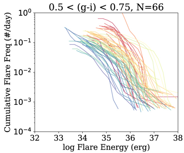
Figure 7. from The Evolution of Flare Activity with Stellar Age null 2019 APJ 871 241 doi:10.3847/1538-4357/aafb76 https://dx.doi.org/10.3847/1538-4357/aafb76 © 2019. The American Astronomical Society.
