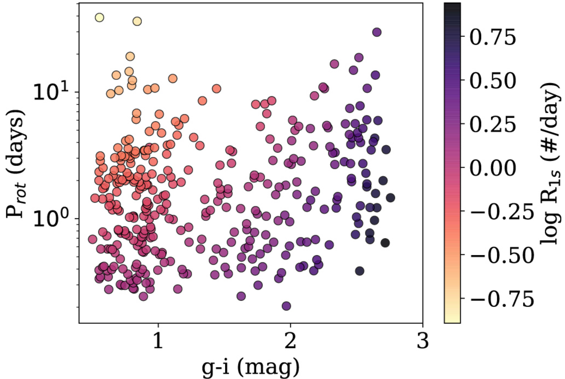
Figure 6. from The Evolution of Flare Activity with Stellar Age null 2019 APJ 871 241 doi:10.3847/1538-4357/aafb76 https://dx.doi.org/10.3847/1538-4357/aafb76 © 2019. The American Astronomical Society.
