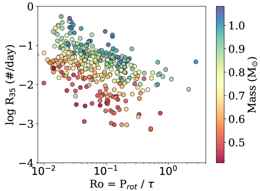
Figure 5. from The Evolution of Flare Activity with Stellar Age null 2019 APJ 871 241 doi:10.3847/1538-4357/aafb76 https://dx.doi.org/10.3847/1538-4357/aafb76 © 2019. The American Astronomical Society.
