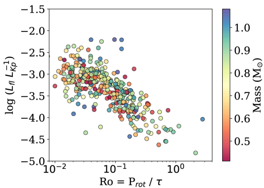
Figure 4. from The Evolution of Flare Activity with Stellar Age null 2019 APJ 871 241 doi:10.3847/1538-4357/aafb76 https://dx.doi.org/10.3847/1538-4357/aafb76 © 2019. The American Astronomical Society.
