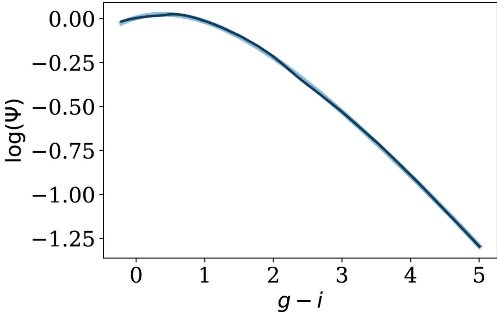
Figure 3. from The Evolution of Flare Activity with Stellar Age null 2019 APJ 871 241 doi:10.3847/1538-4357/aafb76 https://dx.doi.org/10.3847/1538-4357/aafb76 © 2019. The American Astronomical Society.
