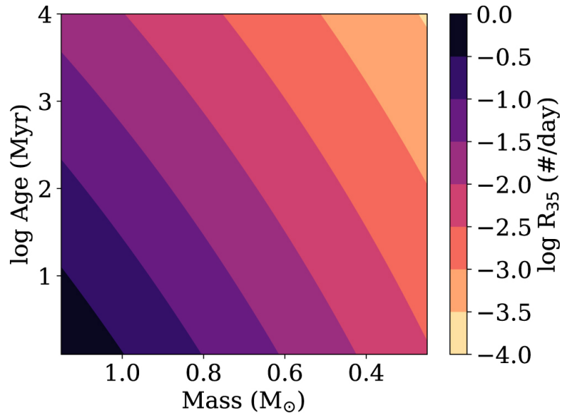
Figure 11. from The Evolution of Flare Activity with Stellar Age null 2019 APJ 871 241 doi:10.3847/1538-4357/aafb76 https://dx.doi.org/10.3847/1538-4357/aafb76 © 2019. The American Astronomical Society.
