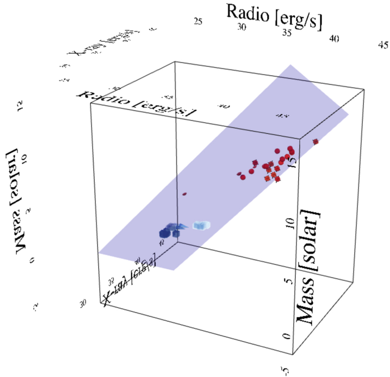
Figure 7. from The Fundamental Plane of Black Hole Accretion and Its Use as a Black Hole-Mass Estimator null 2019 APJ 871 80 doi:10.3847/1538-4357/aaf6b9 https://dx.doi.org/10.3847/1538-4357/aaf6b9 © 2019. The American Astronomical Society. All rights reserved.
