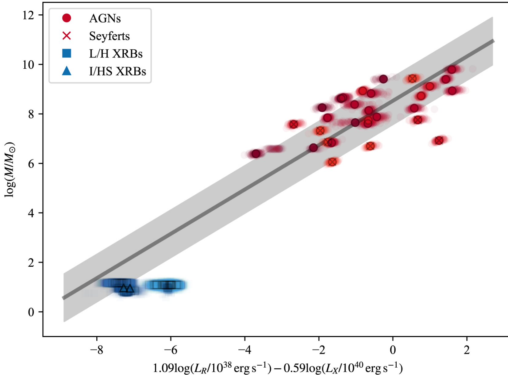
Figure 6. from The Fundamental Plane of Black Hole Accretion and Its Use as a Black Hole-Mass Estimator null 2019 APJ 871 80 doi:10.3847/1538-4357/aaf6b9 https://dx.doi.org/10.3847/1538-4357/aaf6b9 © 2019. The American Astronomical Society. All rights reserved.
