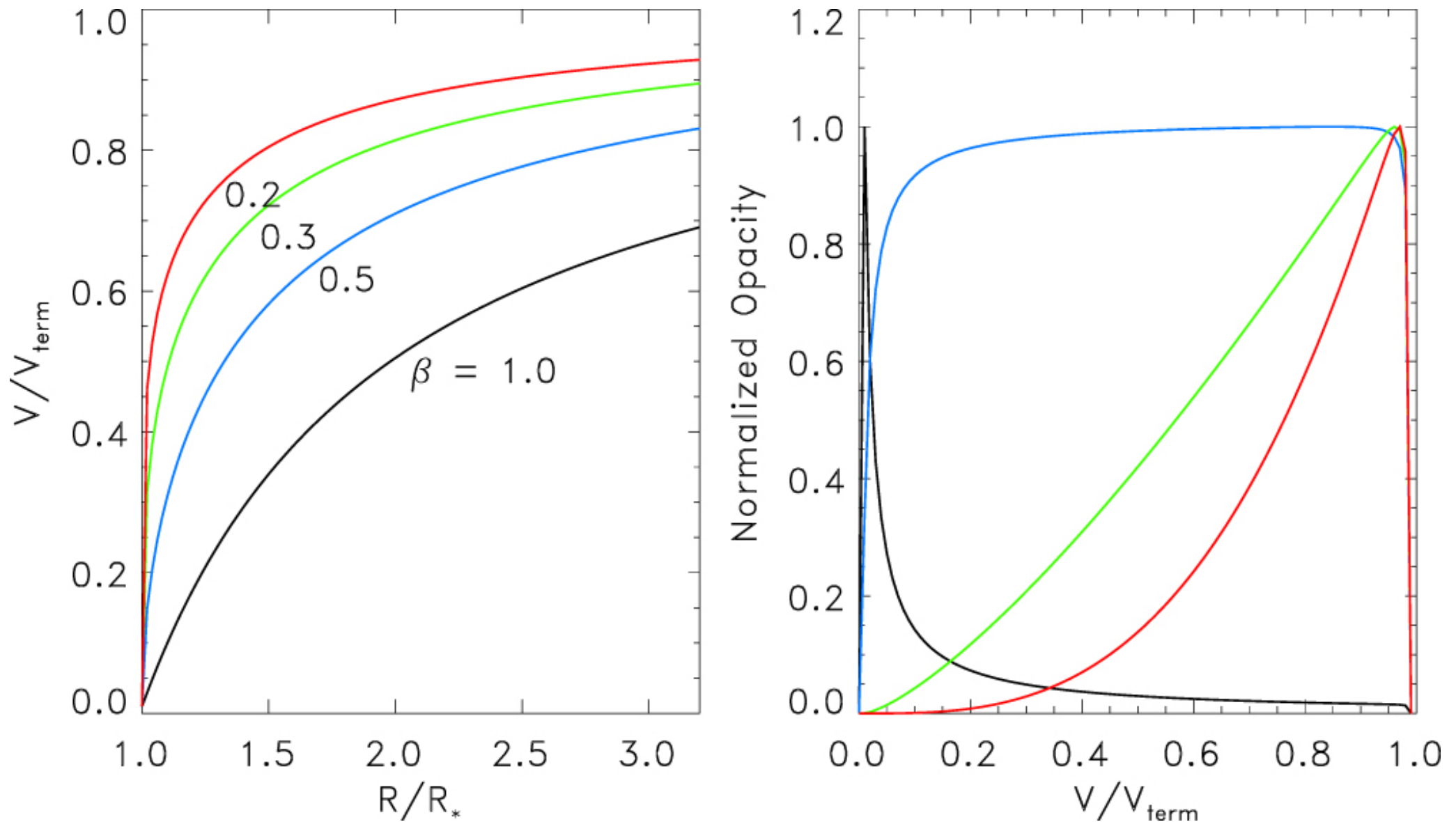
Figure 6. from HST/GHRS Observations of Cool, Low-gravity Stars. VI. Mass-loss Rates and Wind Parameters for M Giants null 2018 APJ 869 1 doi:10.3847/1538-4357/aaf0a0 https://dx.doi.org/10.3847/1538-4357/aaf0a0 © 2018. The American Astronomical Society. All rights reserved.
