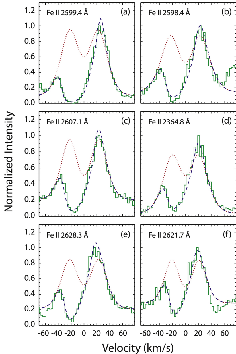
Figure 5. from HST/GHRS Observations of Cool, Low-gravity Stars. VI. Mass-loss Rates and Wind Parameters for M Giants null 2018 APJ 869 1 doi:10.3847/1538-4357/aaf0a0 https://dx.doi.org/10.3847/1538-4357/aaf0a0 © 2018. The American Astronomical Society. All rights reserved.
