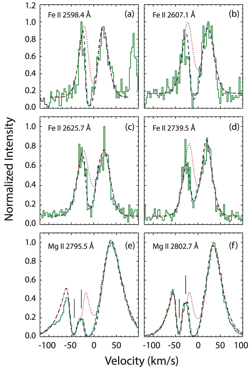
Figure 4. from HST/GHRS Observations of Cool, Low-gravity Stars. VI. Mass-loss Rates and Wind Parameters for M Giants null 2018 APJ 869 1 doi:10.3847/1538-4357/aaf0a0 https://dx.doi.org/10.3847/1538-4357/aaf0a0
