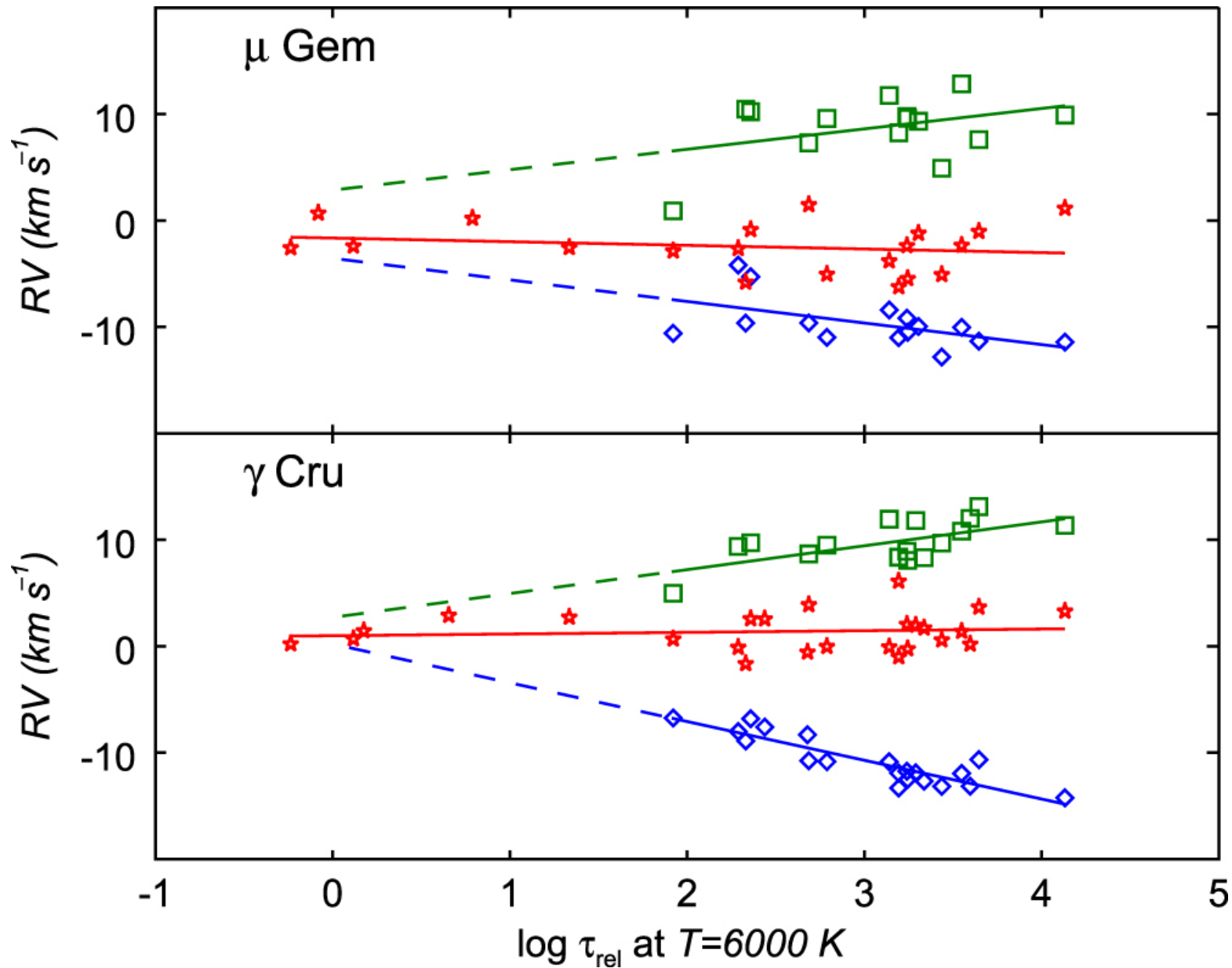
Figure 3. from HST/GHRS Observations of Cool, Low-gravity Stars. VI. Mass-loss Rates and Wind Parameters for M Giants null 2018 APJ 869 1 doi:10.3847/1538-4357/aaf0a0 https://dx.doi.org/10.3847/1538-4357/aaf0a0 © 2018. The American Astronomical Society. All rights reserved.
