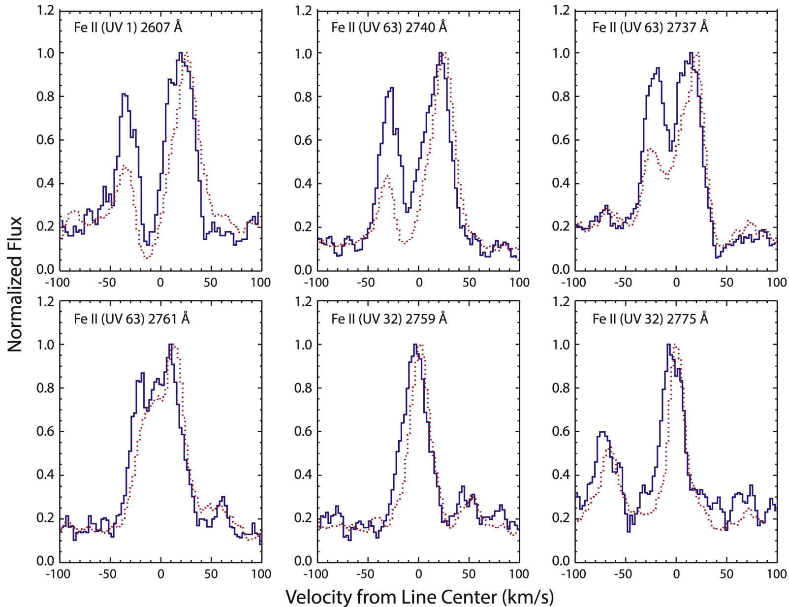
Figure 2. from HST/GHRS Observations of Cool, Low-gravity Stars. VI. Mass-loss Rates and Wind Parameters for M Giants null 2018 APJ 869 1 doi:10.3847/1538-4357/aaf0a0 https://dx.doi.org/10.3847/1538-4357/aaf0a0
