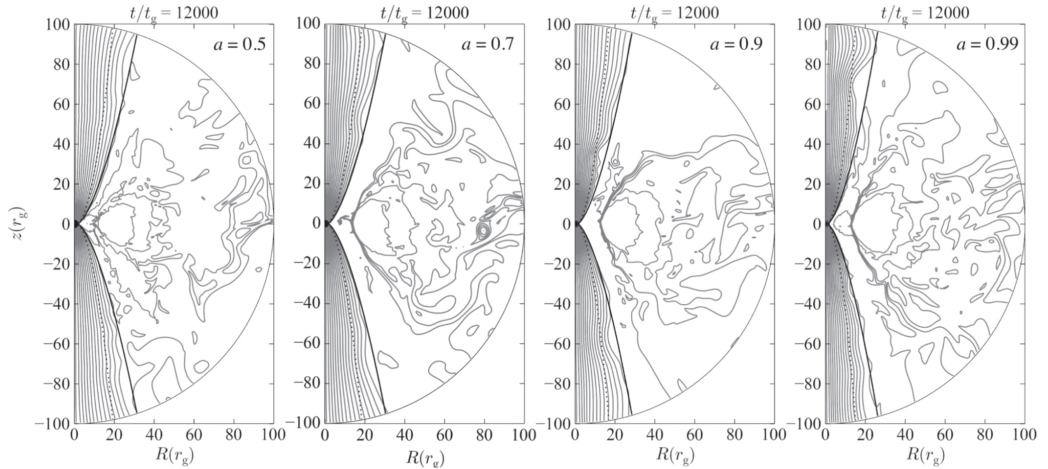
Figure 9. from Parabolic Jets from the Spinning Black Hole in M87 null 2018 APJ 868 146 doi:10.3847/1538-4357/aaeb2d https://dx.doi.org/10.3847/1538-4357/aaeb2d © 2018. The American Astronomical Society. All rights reserved.
