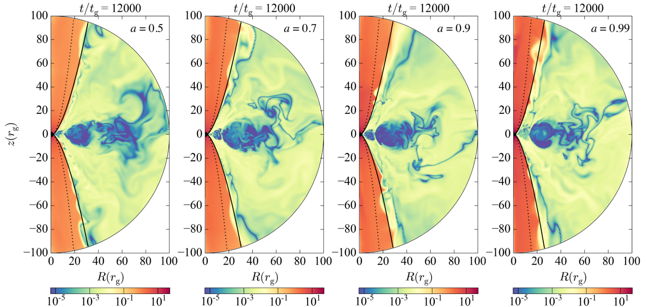
Figure 8. from Parabolic Jets from the Spinning Black Hole in M87 null 2018 APJ 868 146 doi:10.3847/1538-4357/aaeb2d https://dx.doi.org/10.3847/1538-4357/aaeb2d © 2018. The American Astronomical Society. All rights reserved.
