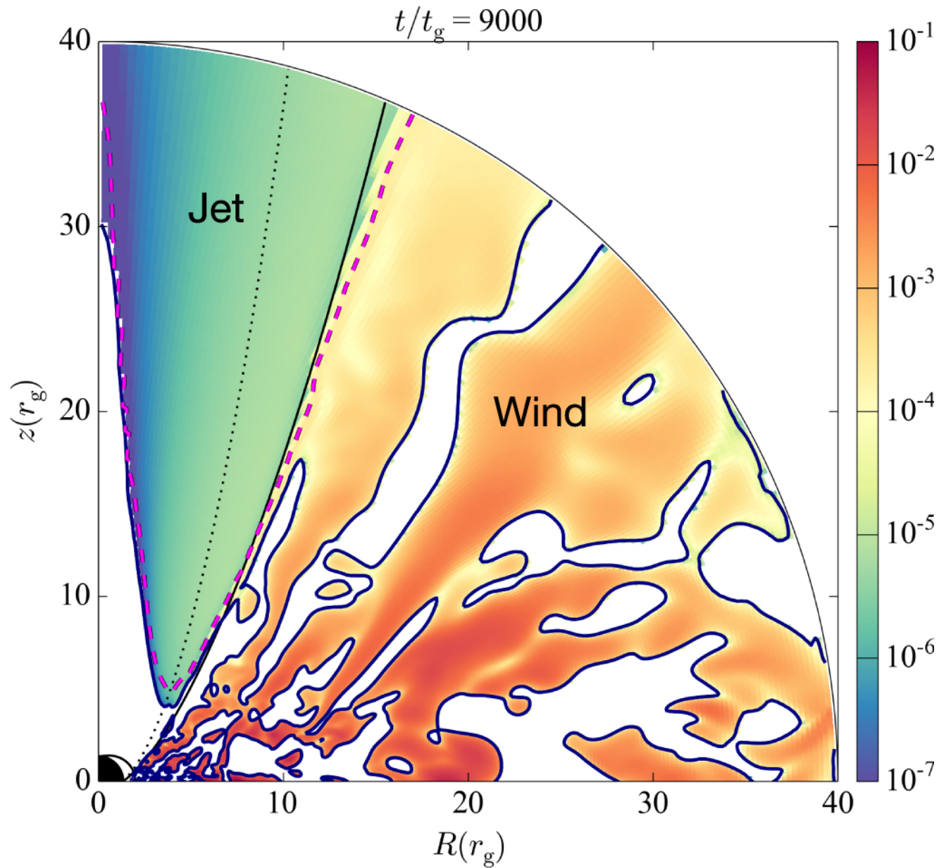
Figure 7. from Parabolic Jets from the Spinning Black Hole in M87 null 2018 APJ 868 146 doi:10.3847/1538-4357/aaeb2d https://dx.doi.org/10.3847/1538-4357/aaeb2d © 2018. The American Astronomical Society. All rights reserved.
