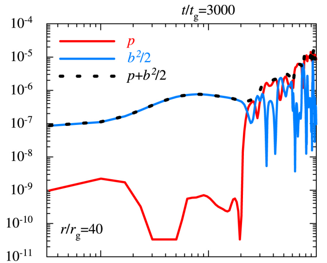
Figure 6. from Parabolic Jets from the Spinning Black Hole in M87 null 2018 APJ 868 146 doi:10.3847/1538-4357/aaeb2d https://dx.doi.org/10.3847/1538-4357/aaeb2d © 2018. The American Astronomical Society. All rights reserved.
