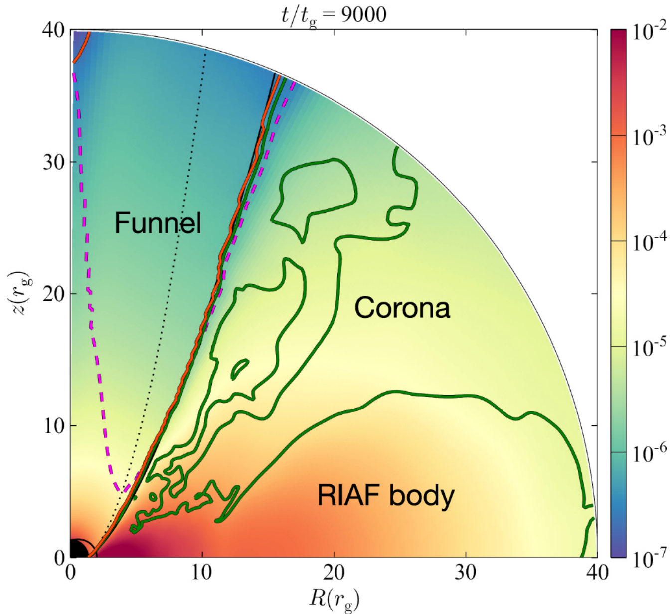
Figure 5. from Parabolic Jets from the Spinning Black Hole in M87 null 2018 APJ 868 146 doi:10.3847/1538-4357/aaeb2d https://dx.doi.org/10.3847/1538-4357/aaeb2d © 2018. The American Astronomical Society. All rights reserved.
