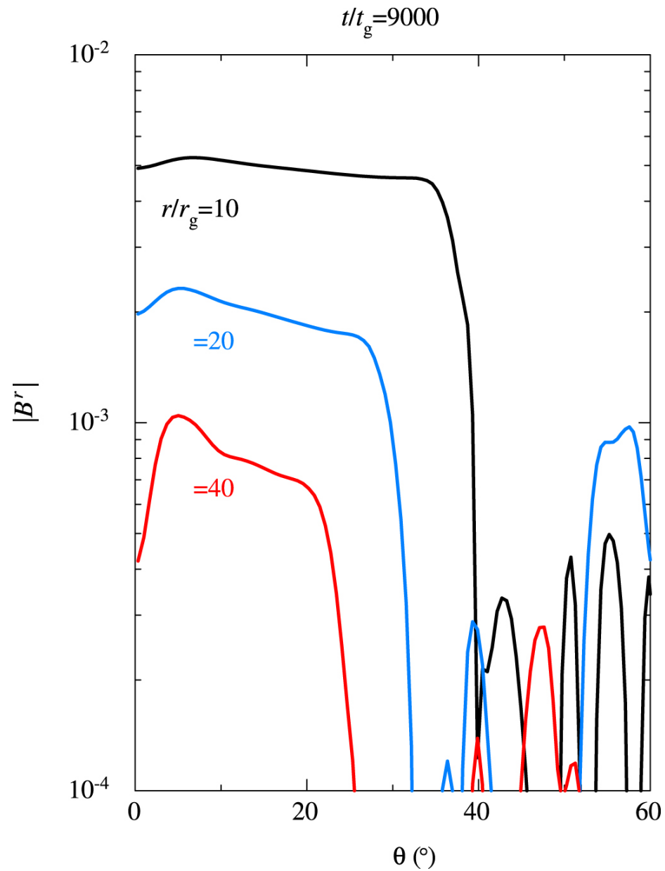
Figure 4. from Parabolic Jets from the Spinning Black Hole in M87 null 2018 APJ 868 146 doi:10.3847/1538-4357/aaeb2d https://dx.doi.org/10.3847/1538-4357/aaeb2d © 2018. The American Astronomical Society. All rights reserved.
