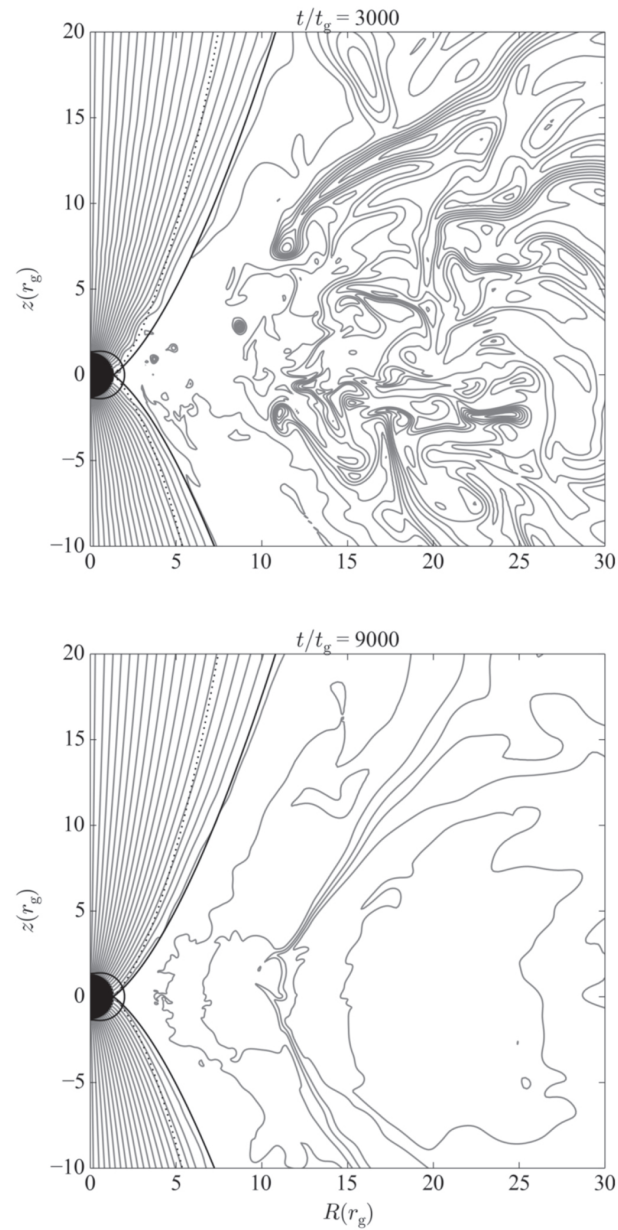
Figure 3. from Parabolic Jets from the Spinning Black Hole in M87 null 2018 APJ 868 146 doi:10.3847/1538-4357/aaeb2d https://dx.doi.org/10.3847/1538-4357/aaeb2d © 2018. The American Astronomical Society. All rights reserved.
