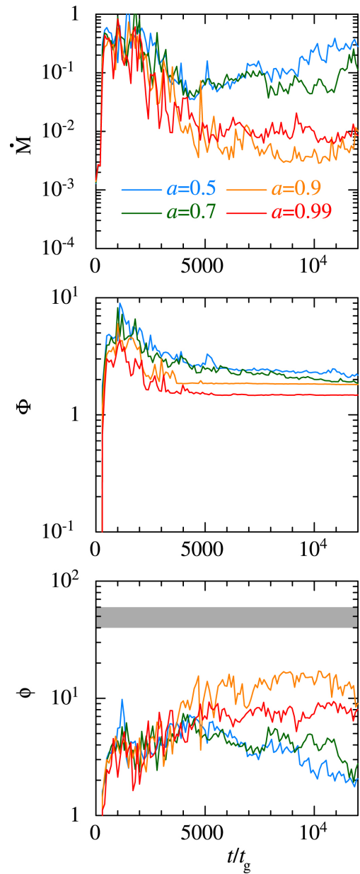
Figure 23. from Parabolic Jets from the Spinning Black Hole in M87 null 2018 APJ 868 146 doi:10.3847/1538-4357/aaeb2d https://dx.doi.org/10.3847/1538-4357/aaeb2d © 2018. The American Astronomical Society. All rights reserved.
