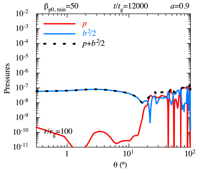
Figure 22. from Parabolic Jets from the Spinning Black Hole in M87 null 2018 APJ 868 146 doi:10.3847/1538-4357/aaeb2d https://dx.doi.org/10.3847/1538-4357/aaeb2d
