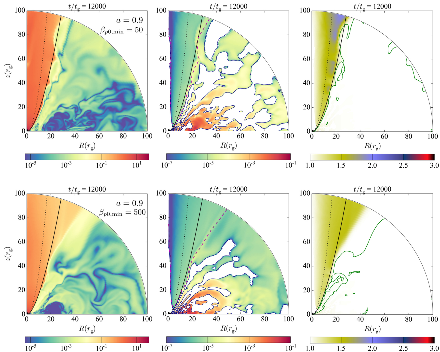
Figure 21. from Parabolic Jets from the Spinning Black Hole in M87 null 2018 APJ 868 146 doi:10.3847/1538-4357/aaeb2d https://dx.doi.org/10.3847/1538-4357/aaeb2d © 2018. The American Astronomical Society. All rights reserved.
