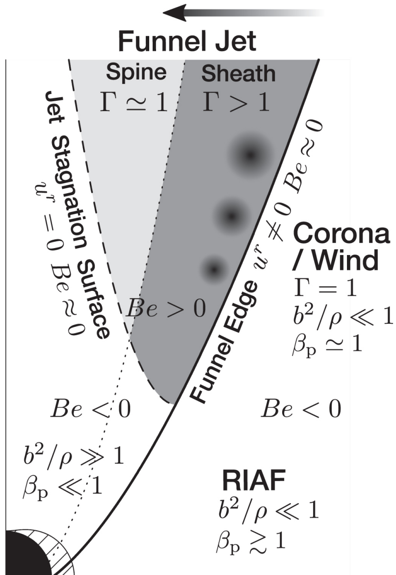
Figure 20. from Parabolic Jets from the Spinning Black Hole in M87 null 2018 APJ 868 146 doi:10.3847/1538-4357/aaeb2d https://dx.doi.org/10.3847/1538-4357/aaeb2d © 2018. The American Astronomical Society. All rights reserved.
