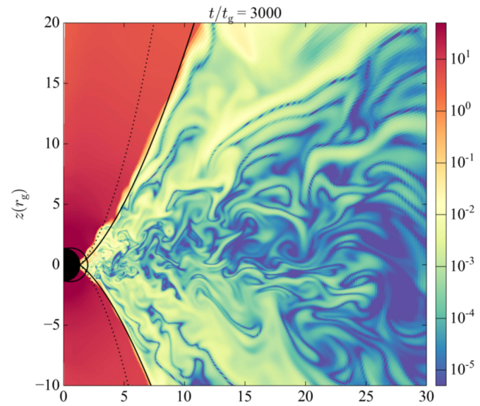
Figure 2. from Parabolic Jets from the Spinning Black Hole in M87 null 2018 APJ 868 146 doi:10.3847/1538-4357/aaeb2d https://dx.doi.org/10.3847/1538-4357/aaeb2d © 2018. The American Astronomical Society. All rights reserved.
