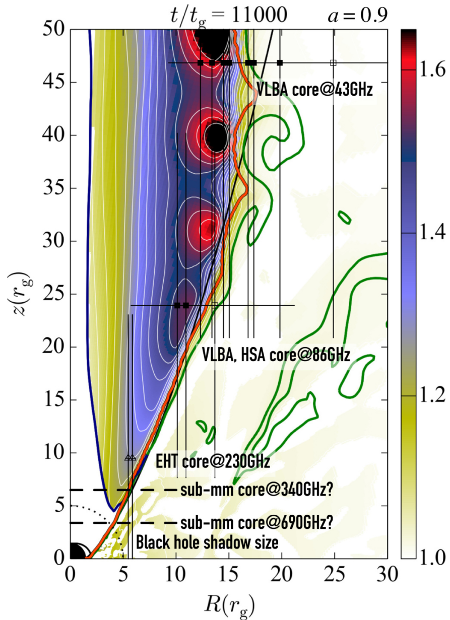
Figure 19. from Parabolic Jets from the Spinning Black Hole in M87 null 2018 APJ 868 146 doi:10.3847/1538-4357/aaeb2d https://dx.doi.org/10.3847/1538-4357/aaeb2d © 2018. The American Astronomical Society. All rights reserved.
