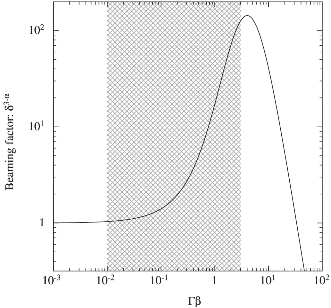
Figure 18. from Parabolic Jets from the Spinning Black Hole in M87 null 2018 APJ 868 146 doi:10.3847/1538-4357/aaeb2d https://dx.doi.org/10.3847/1538-4357/aaeb2d © 2018. The American Astronomical Society. All rights reserved.
