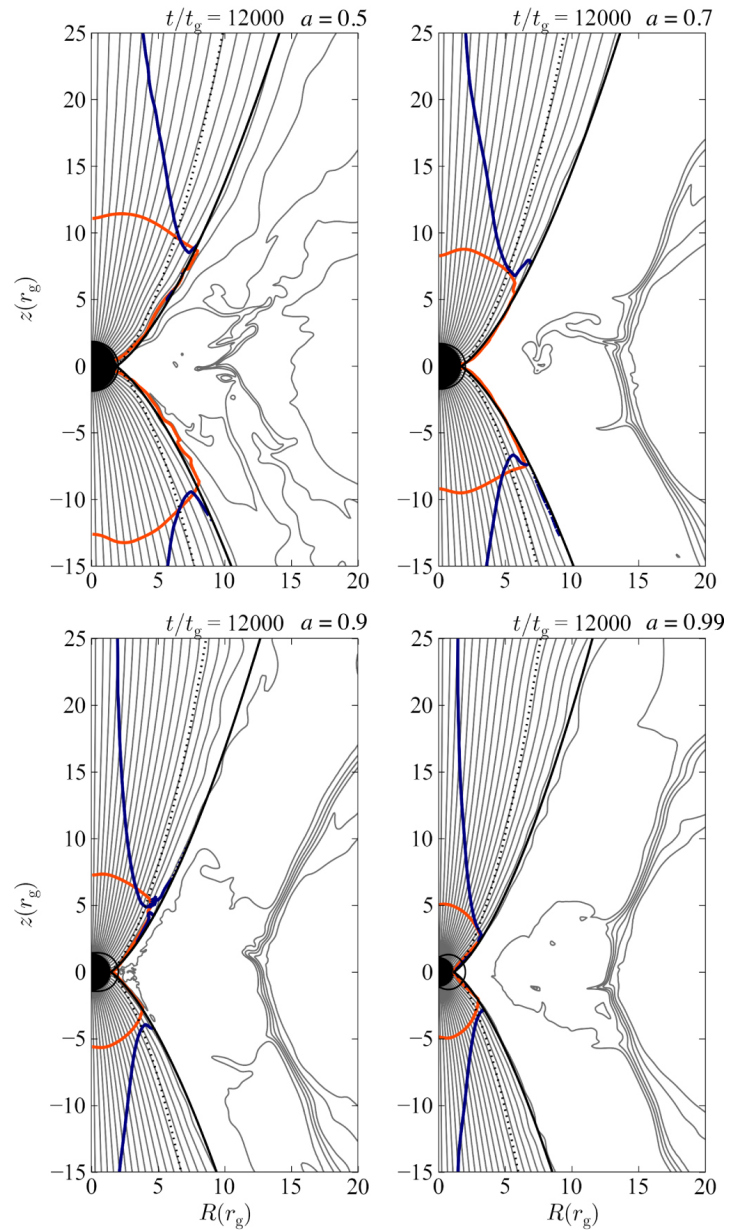
Figure 14. from Parabolic Jets from the Spinning Black Hole in M87 null 2018 APJ 868 146 doi:10.3847/1538-4357/aaeb2d https://dx.doi.org/10.3847/1538-4357/aaeb2d © 2018. The American Astronomical Society. All rights reserved.
