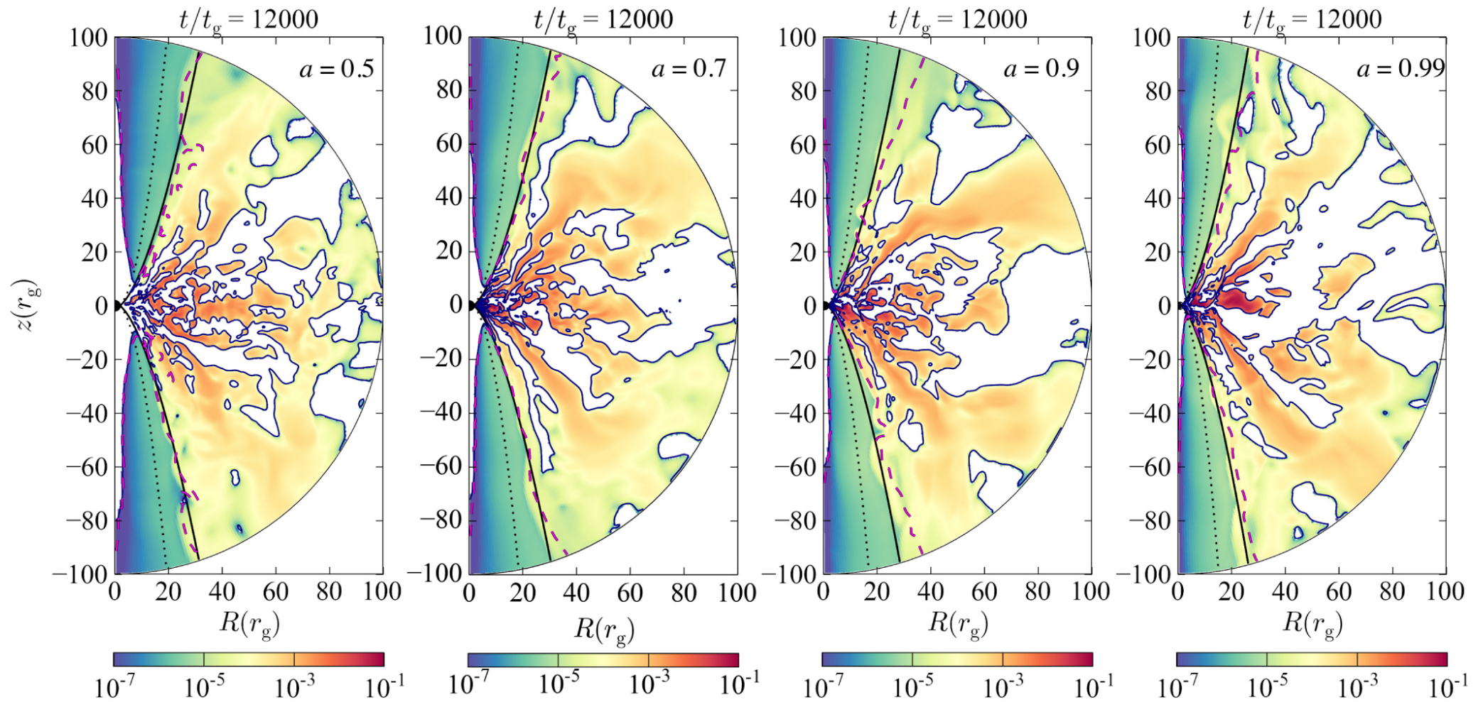
Figure 11. from Parabolic Jets from the Spinning Black Hole in M87 null 2018 APJ 868 146 doi:10.3847/1538-4357/aaeb2d https://dx.doi.org/10.3847/1538-4357/aaeb2d © 2018. The American Astronomical Society. All rights reserved.
