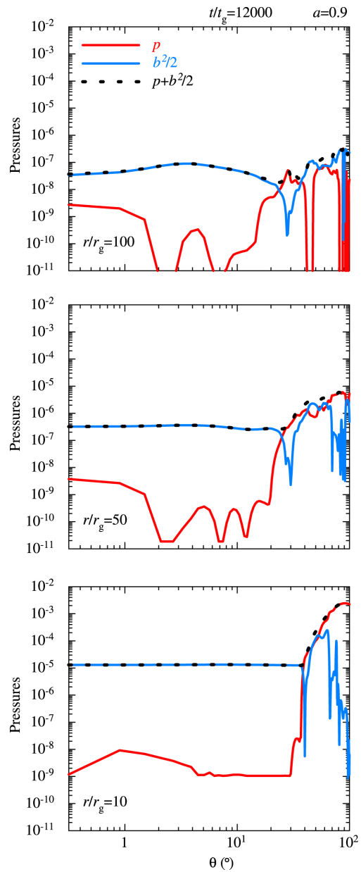
Figure 10. from Parabolic Jets from the Spinning Black Hole in M87 null 2018 APJ 868 146 doi:10.3847/1538-4357/aaeb2d https://dx.doi.org/10.3847/1538-4357/aaeb2d © 2018. The American Astronomical Society. All rights reserved.
