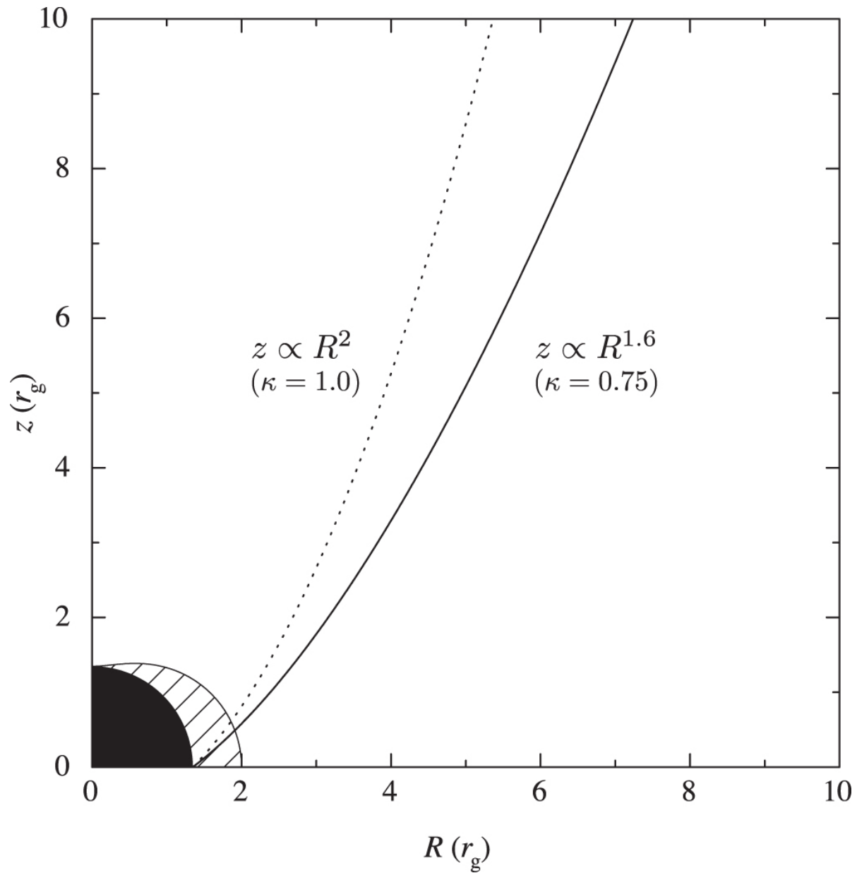
Figure 1. from Parabolic Jets from the Spinning Black Hole in M87 null 2018 APJ 868 146 doi:10.3847/1538-4357/aaeb2d https://dx.doi.org/10.3847/1538-4357/aaeb2d © 2018. The American Astronomical Society. All rights reserved.
