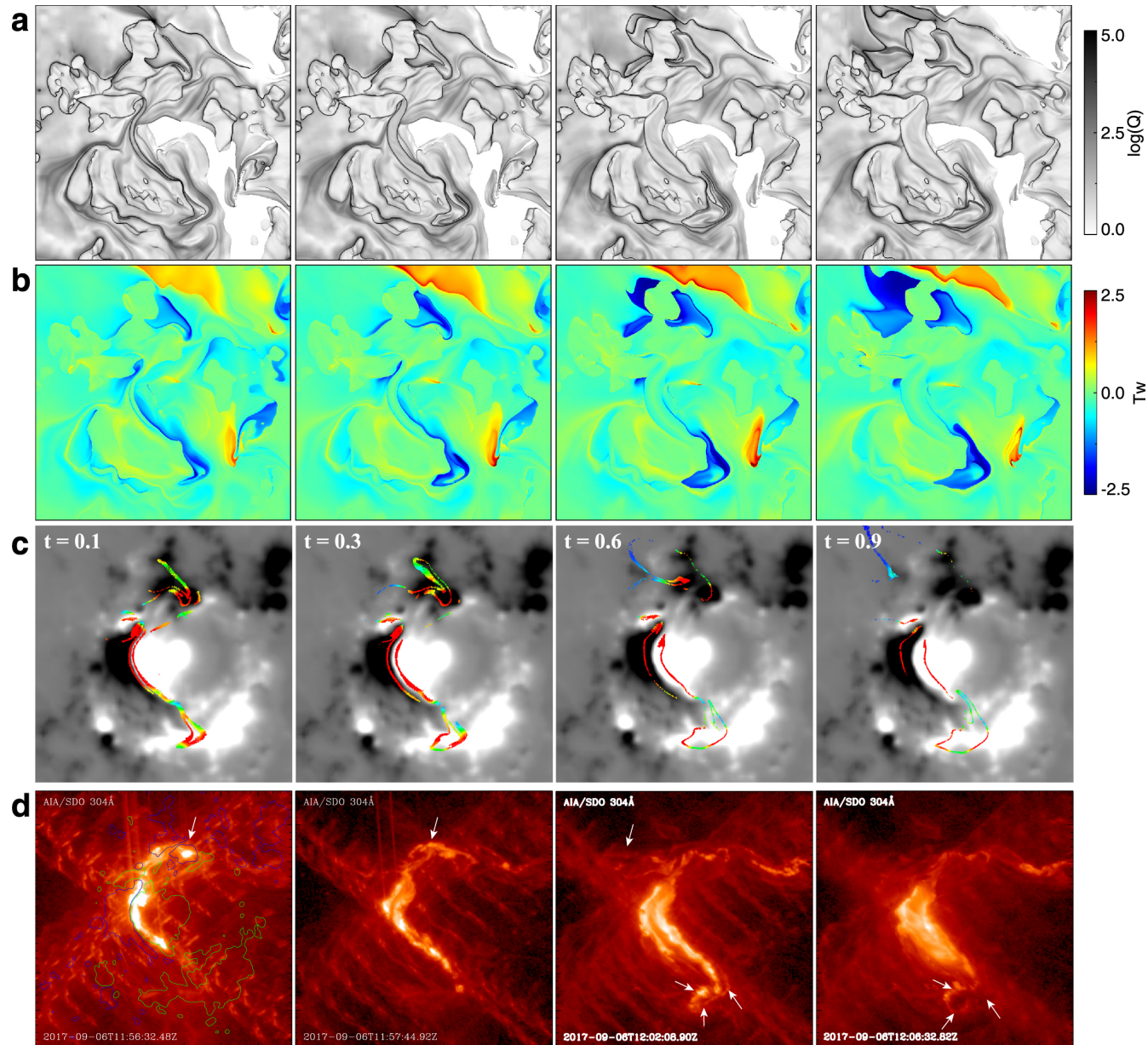
Figure 9. from Magnetohydrodynamic Simulation of the X9.3 Flare on 2017 September 6: Evolving Magnetic Topology null 2018 APJ 869 13 doi:10.3847/1538-4357/aaeacc https://dx.doi.org/10.3847/1538-4357/aaeacc © 2018. The American Astronomical Society. All rights reserved.
