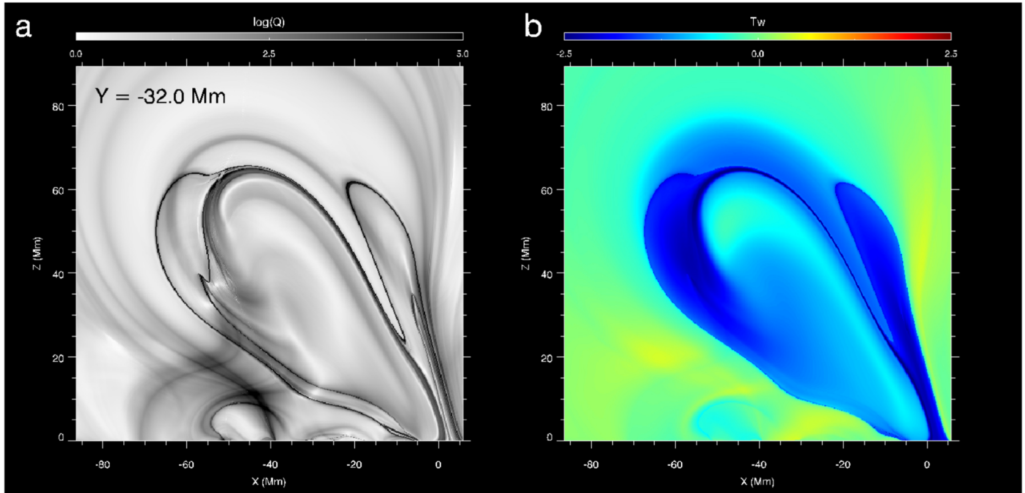
Figure 8. from Magnetohydrodynamic Simulation of the X9.3 Flare on 2017 September 6: Evolving Magnetic Topology null 2018 APJ 869 13 doi:10.3847/1538-4357/aaeacc https://dx.doi.org/10.3847/1538-4357/aaeacc © 2018. The American Astronomical Society. All rights reserved.
