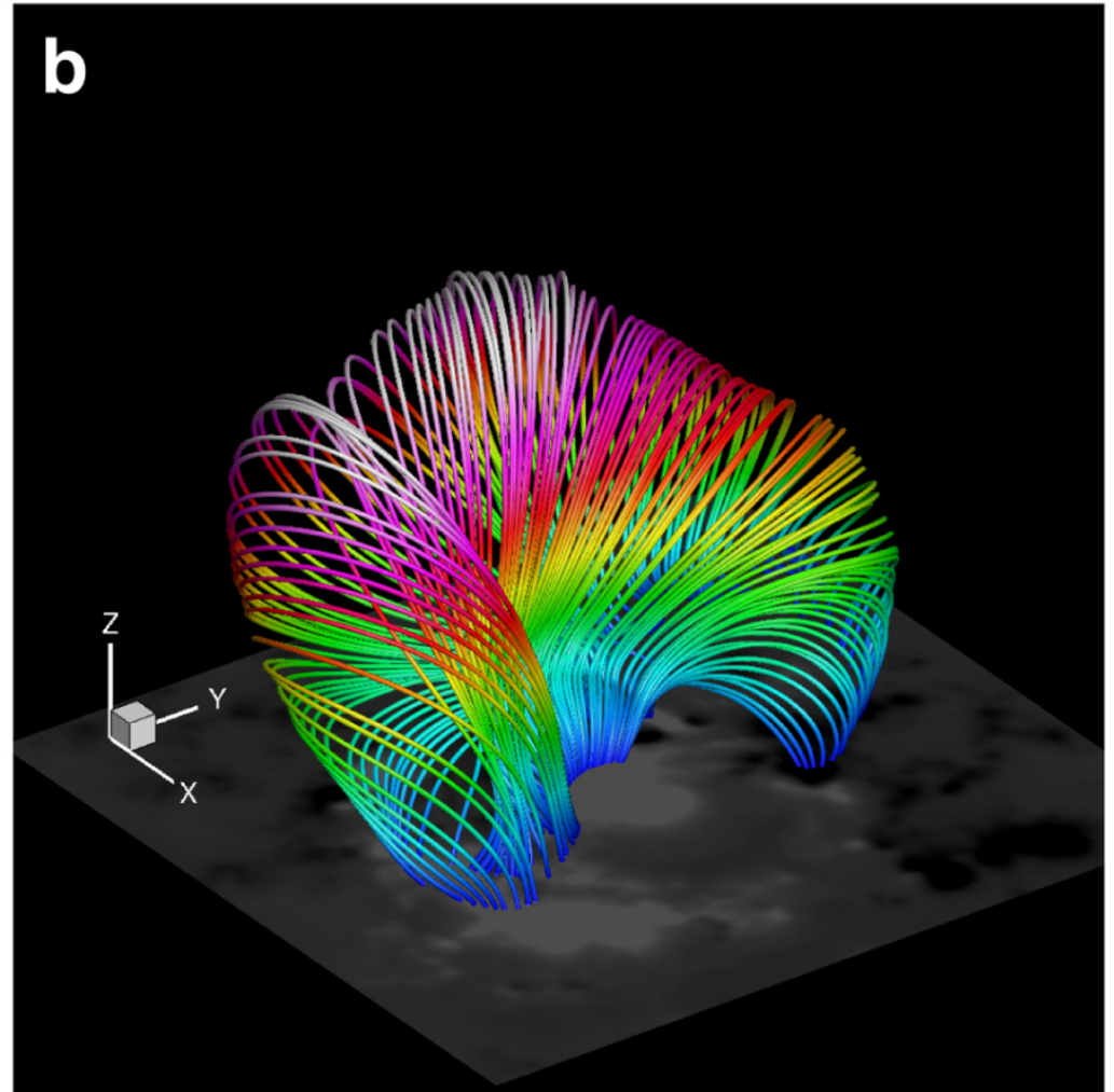
Figure 7. from Magnetohydrodynamic Simulation of the X9.3 Flare on 2017 September 6: Evolving Magnetic Topology null 2018 APJ 869 13 doi:10.3847/1538-4357/aaeacc https://dx.doi.org/10.3847/1538-4357/aaeacc © 2018. The American Astronomical Society. All rights reserved.
