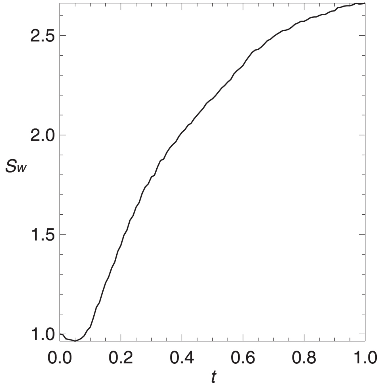
Figure 6. from Magnetohydrodynamic Simulation of the X9.3 Flare on 2017 September 6: Evolving Magnetic Topology null 2018 APJ 869 13 doi:10.3847/1538-4357/aaeacc https://dx.doi.org/10.3847/1538-4357/aaeacc © 2018. The American Astronomical Society. All rights reserved.
