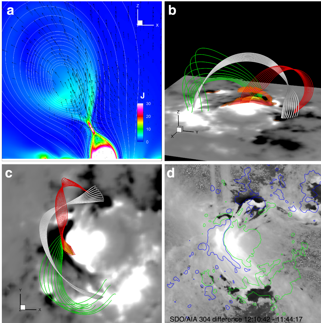
Figure 5. from Magnetohydrodynamic Simulation of the X9.3 Flare on 2017 September 6: Evolving Magnetic Topology null 2018 APJ 869 13 doi:10.3847/1538-4357/aaeacc https://dx.doi.org/10.3847/1538-4357/aaeacc © 2018. The American Astronomical Society. All rights reserved.
