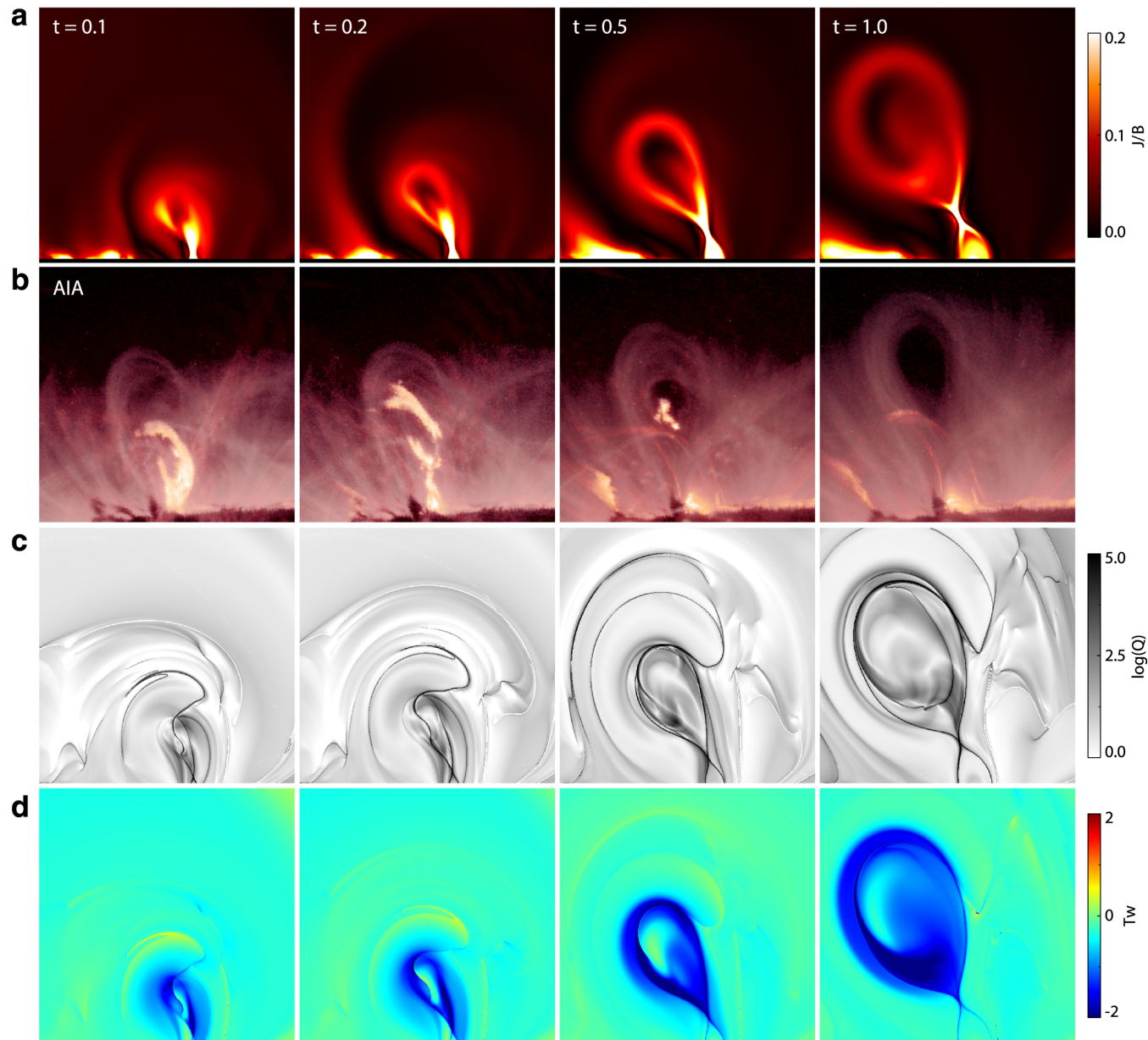
Figure 4. from Magnetohydrodynamic Simulation of the X9.3 Flare on 2017 September 6: Evolving Magnetic Topology null 2018 APJ 869 13 doi:10.3847/1538-4357/aaeacc https://dx.doi.org/10.3847/1538-4357/aaeacc © 2018. The American Astronomical Society. All rights reserved.
