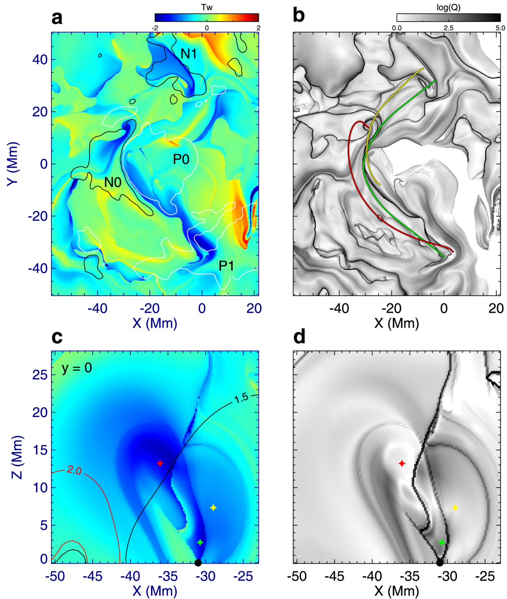
Figure 3. from Magnetohydrodynamic Simulation of the X9.3 Flare on 2017 September 6: Evolving Magnetic Topology null 2018 APJ 869 13 doi:10.3847/1538-4357/aaeacc https://dx.doi.org/10.3847/1538-4357/aaeacc © 2018. The American Astronomical Society. All rights reserved.
