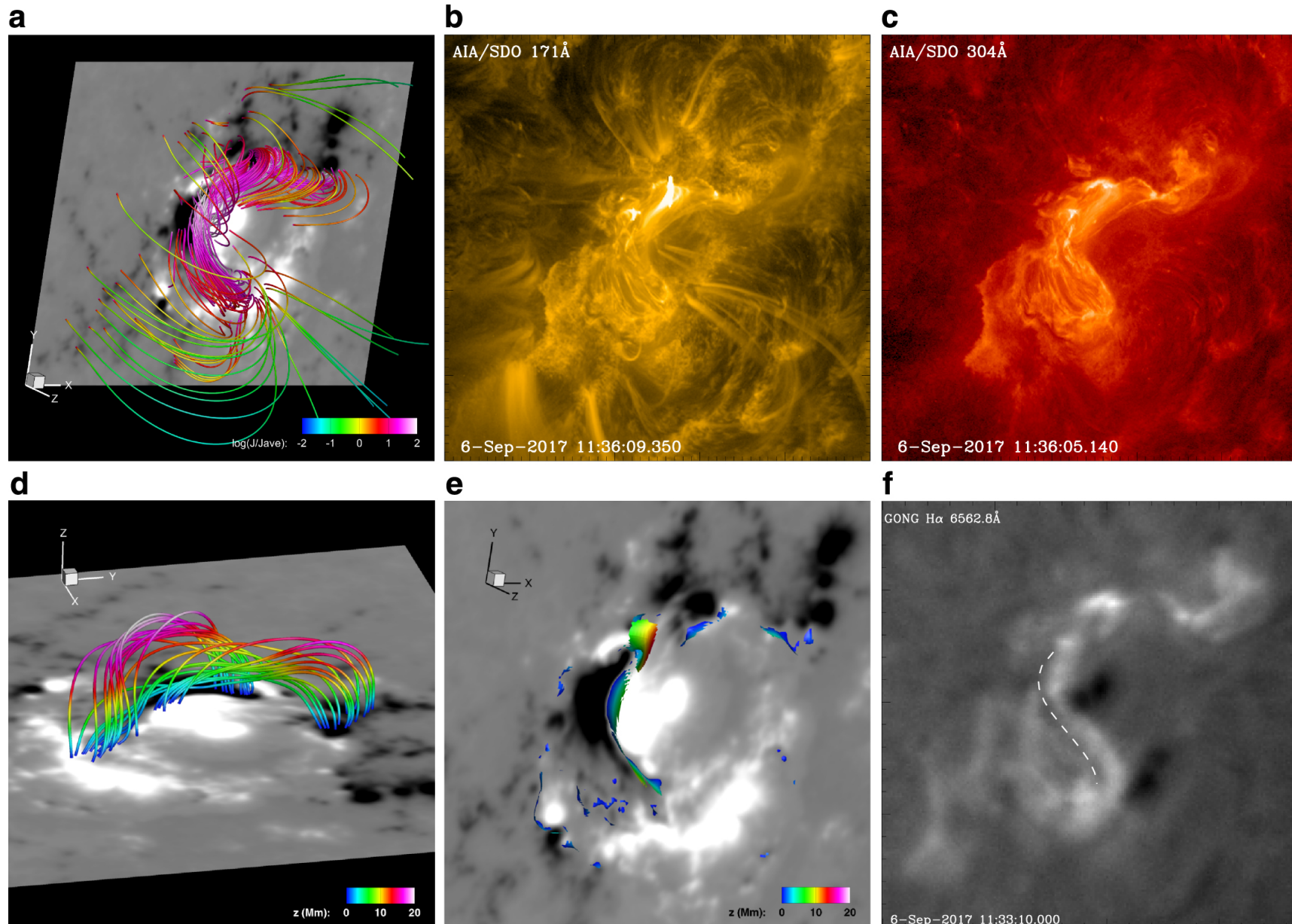
Figure 2. from Magnetohydrodynamic Simulation of the X9.3 Flare on 2017 September 6: Evolving Magnetic Topology null 2018 APJ 869 13 doi:10.3847/1538-4357/aaeacc https://dx.doi.org/10.3847/1538-4357/aaeacc © 2018. The American Astronomical Society. All rights reserved.
