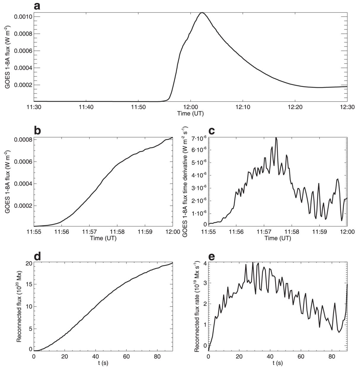
Figure 15. from Magnetohydrodynamic Simulation of the X9.3 Flare on 2017 September 6: Evolving Magnetic Topology null 2018 APJ 869 13 doi:10.3847/1538-4357/aaeacc https://dx.doi.org/10.3847/1538-4357/aaeacc © 2018. The American Astronomical Society. All rights reserved.
