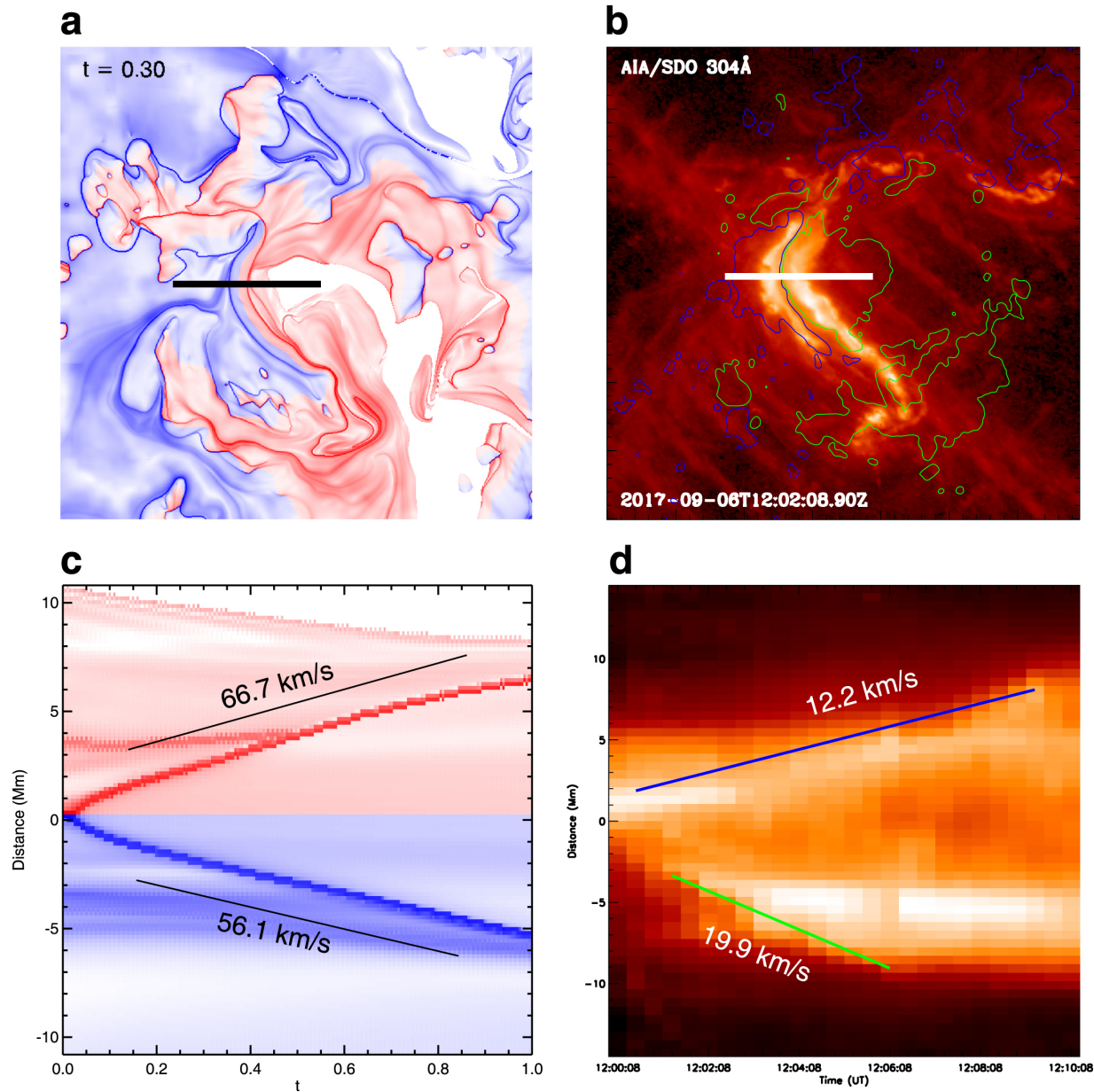
Figure 14. from Magnetohydrodynamic Simulation of the X9.3 Flare on 2017 September 6: Evolving Magnetic Topology null 2018 APJ 869 13 doi:10.3847/1538-4357/aaeacc https://dx.doi.org/10.3847/1538-4357/aaeacc © 2018. The American Astronomical Society. All rights reserved.
