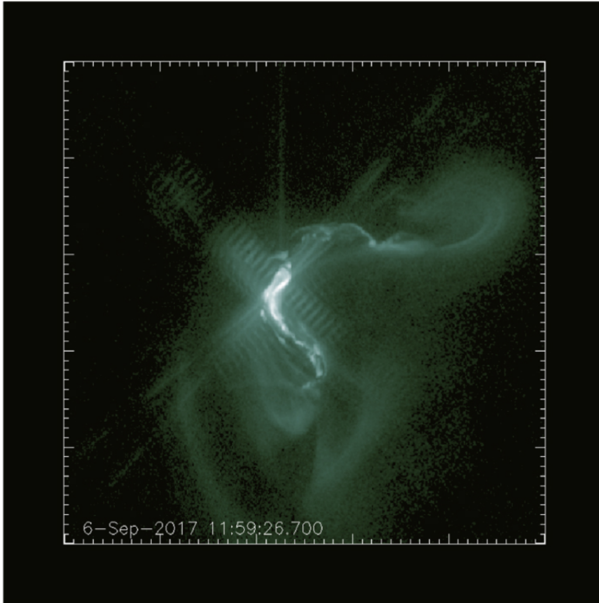
Figure 13. from Magnetohydrodynamic Simulation of the X9.3 Flare on 2017 September 6: Evolving Magnetic Topology null 2018 APJ 869 13 doi:10.3847/1538-4357/aaeacc https://dx.doi.org/10.3847/1538-4357/aaeacc © 2018. The American Astronomical Society. All rights reserved.
