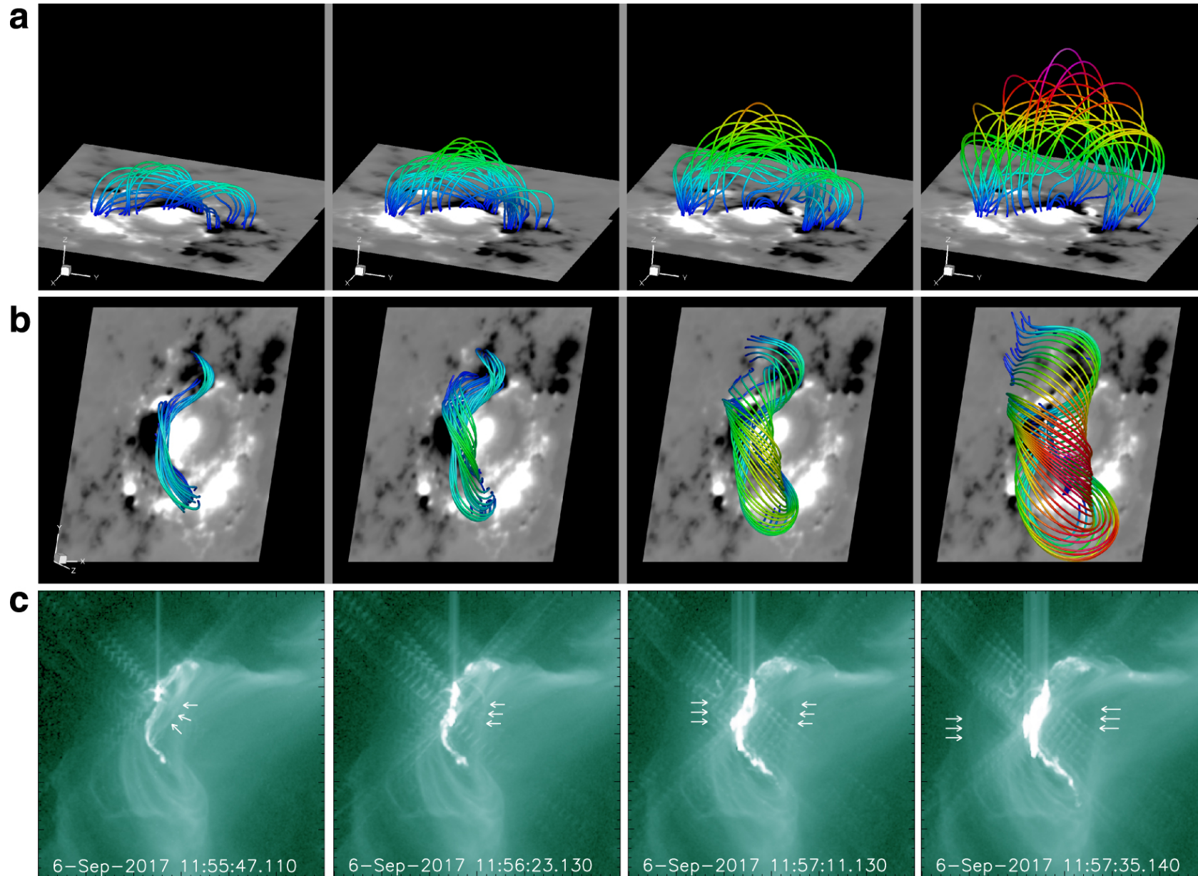
Figure 12. from Magnetohydrodynamic Simulation of the X9.3 Flare on 2017 September 6: Evolving Magnetic Topology null 2018 APJ 869 13 doi:10.3847/1538-4357/aaeacc https://dx.doi.org/10.3847/1538-4357/aaeacc © 2018. The American Astronomical Society. All rights reserved.
