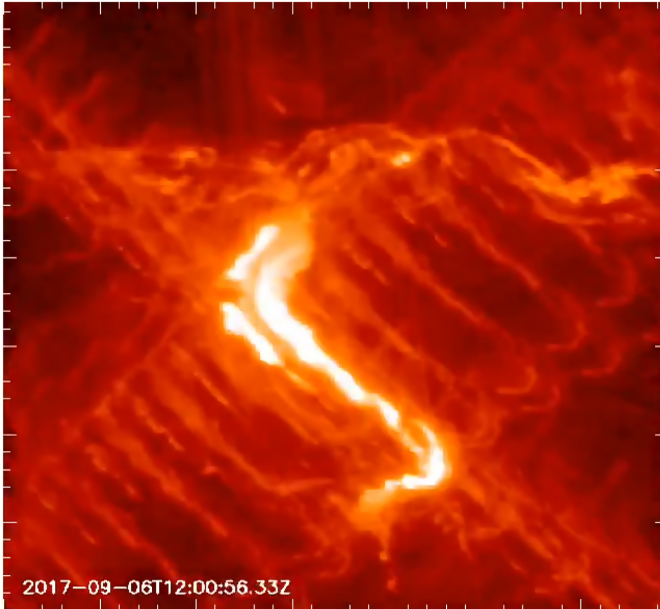
Figure 11. from Magnetohydrodynamic Simulation of the X9.3 Flare on 2017 September 6: Evolving Magnetic Topology null 2018 APJ 869 13 doi:10.3847/1538-4357/aaeacc https://dx.doi.org/10.3847/1538-4357/aaeacc © 2018. The American Astronomical Society. All rights reserved.
