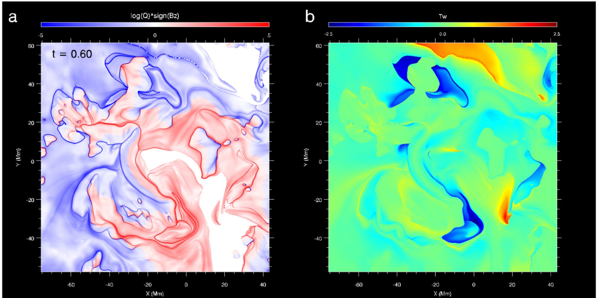
Figure 10. from Magnetohydrodynamic Simulation of the X9.3 Flare on 2017 September 6: Evolving Magnetic Topology null 2018 APJ 869 13 doi:10.3847/1538-4357/aaeacc https://dx.doi.org/10.3847/1538-4357/aaeacc © 2018. The American Astronomical Society. All rights reserved.
