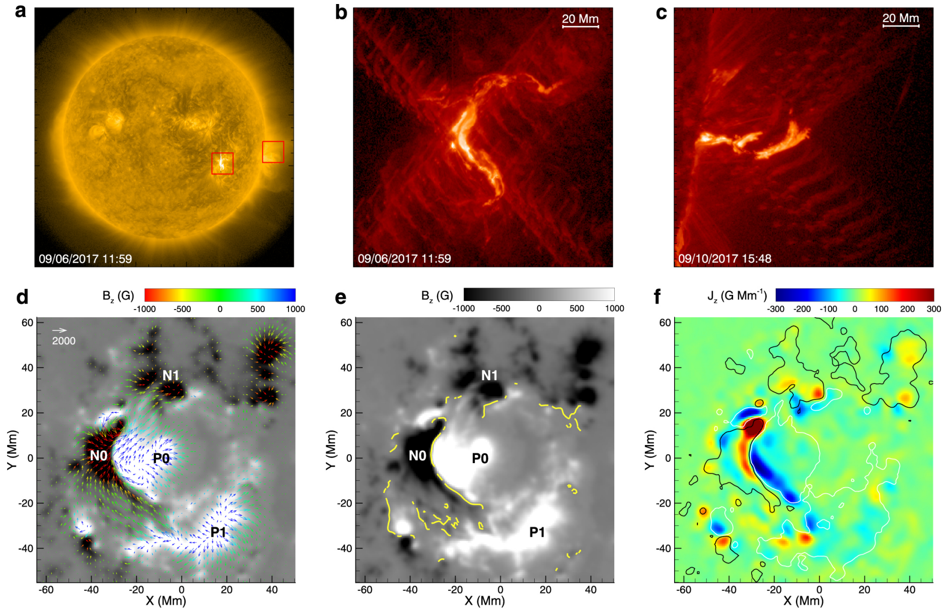
Figure 1. from Magnetohydrodynamic Simulation of the X9.3 Flare on 2017 September 6: Evolving Magnetic Topology null 2018 APJ 869 13 doi:10.3847/1538-4357/aaeacc https://dx.doi.org/10.3847/1538-4357/aaeacc © 2018. The American Astronomical Society. All rights reserved.
