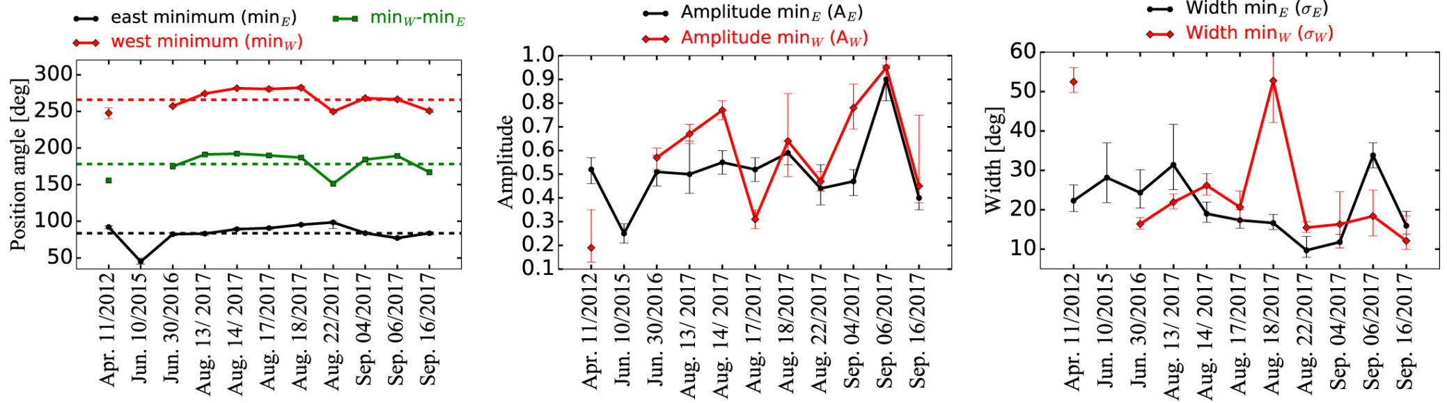
Figure 6. from Variable Outer Disk Shadowing around the Dipper Star RXJ1604.3–2130 null 2018 APJ 868 85 doi:10.3847/1538-4357/aae824 https://dx.doi.org/10.3847/1538-4357/aae824 © 2018. The American Astronomical Society. All rights reserved.
