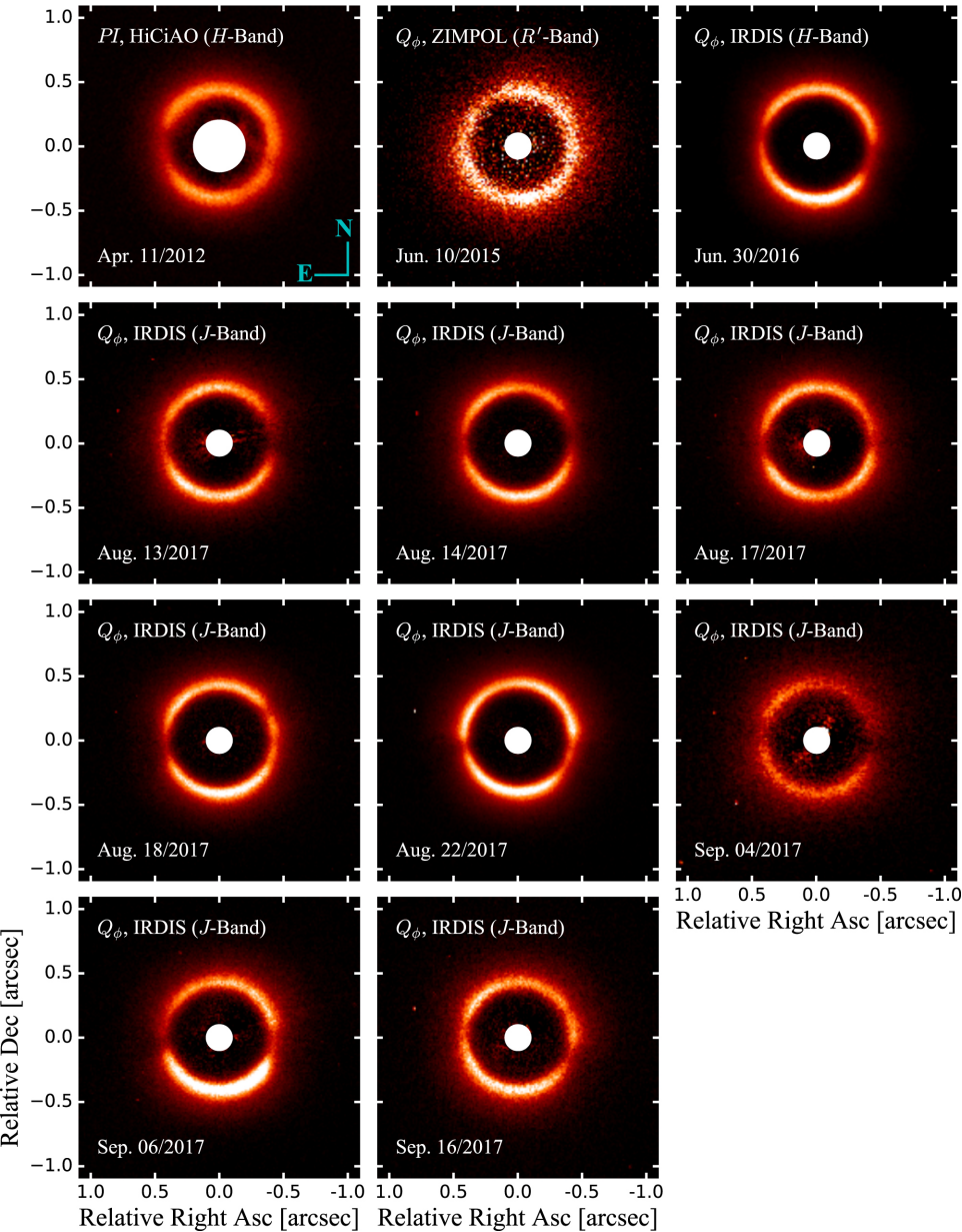
Figure 1. from Variable Outer Disk Shadowing around the Dipper Star RXJ1604.3–2130 null 2018 APJ 868 85 doi:10.3847/1538-4357/aae824 https://dx.doi.org/10.3847/1538-4357/aae824 © 2018. The American Astronomical Society. All rights reserved.
