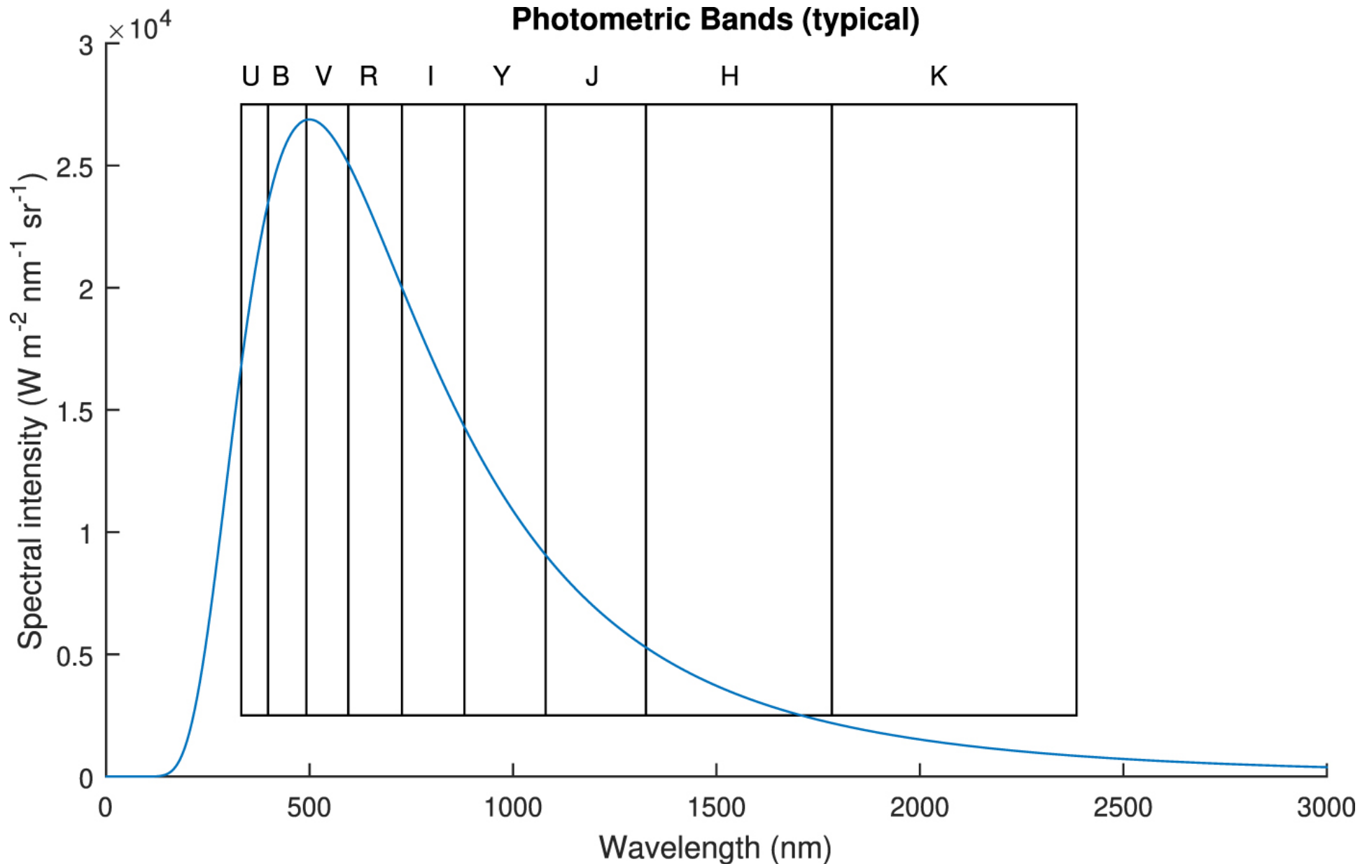
Figure 4. from Optical Detection of Lasers with Near-term Technology at Interstellar Distances null 2018 APJ 867 97 doi:10.3847/1538-4357/aae380 https://dx.doi.org/10.3847/1538-4357/aae380 © 2018. The American Astronomical Society.
